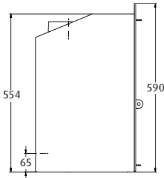
WESTFIRE.UNIQ.35 | INSERT 3-SIDED FRAME WEIGHT: 75 KG
