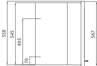
WESTFIRE.UNIQ.32 | INSERT WIDE 4-SIDED FRAME WEIGHT: 110 KG
