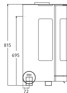
WESTFIRE.UNIQ.36 WESTFIRE.UNIQ.37 COMPACT | WEIGHT: 85 KG
