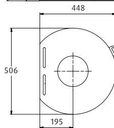
WESTFIRE.UNIQ.46 (FORMERLY UNIQ 18 WITH LOGDOOR) WEIGHT: 90 KG
